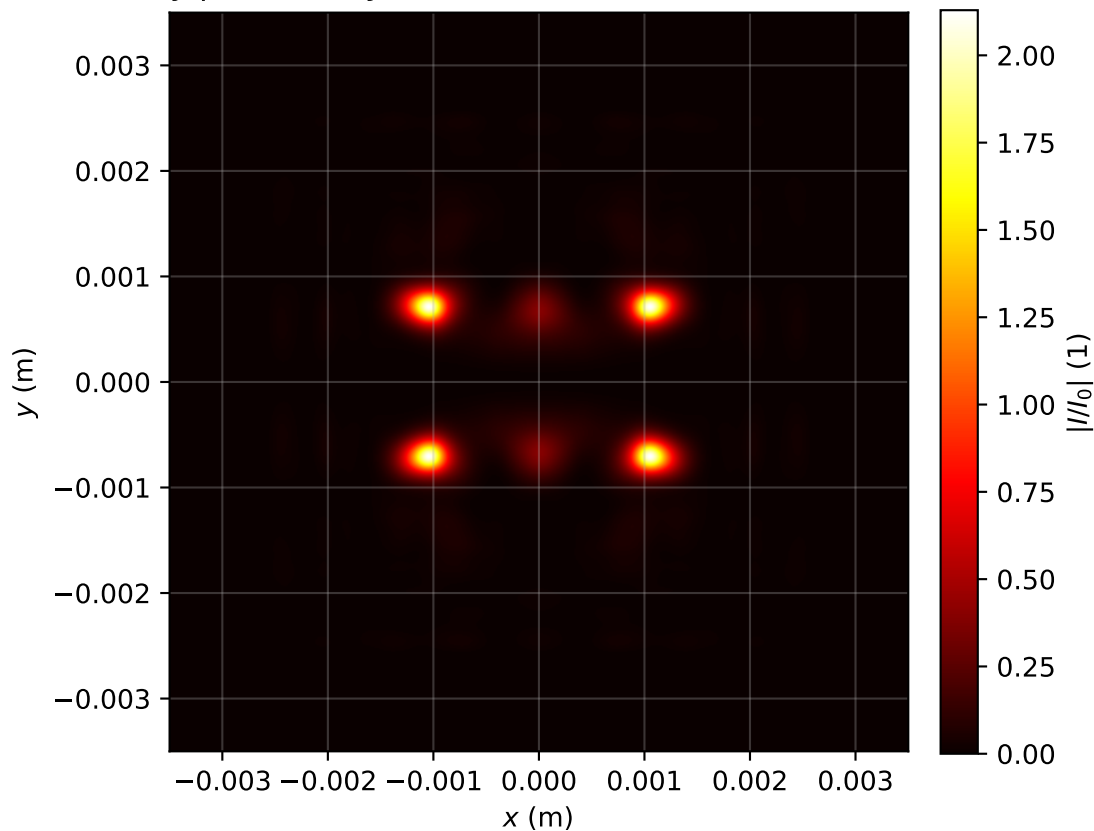
Intensity profile I(x, y, z = 2.309)/I_0 , P_{in}=7.0P_{cr} , artificial time
